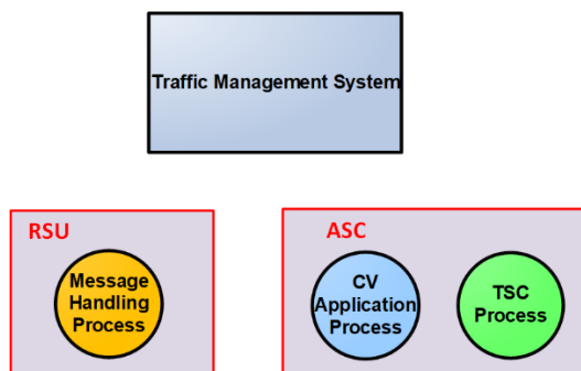
Figure 5 Physical Architecture 1
