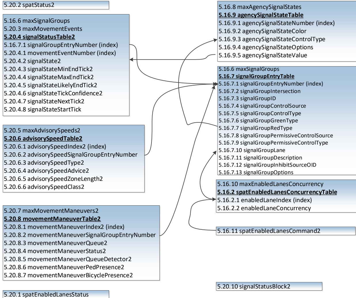
Figure 13 NTCIP 1202 v04 Tables to Provide SPaT Data
