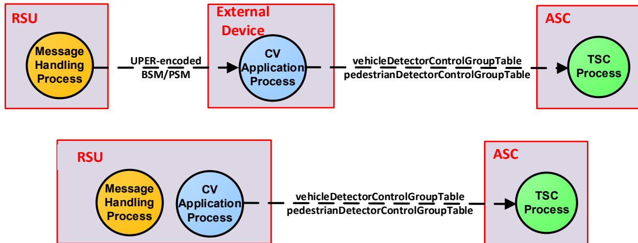
Figure 23 Connected Device Detector - Profile B
