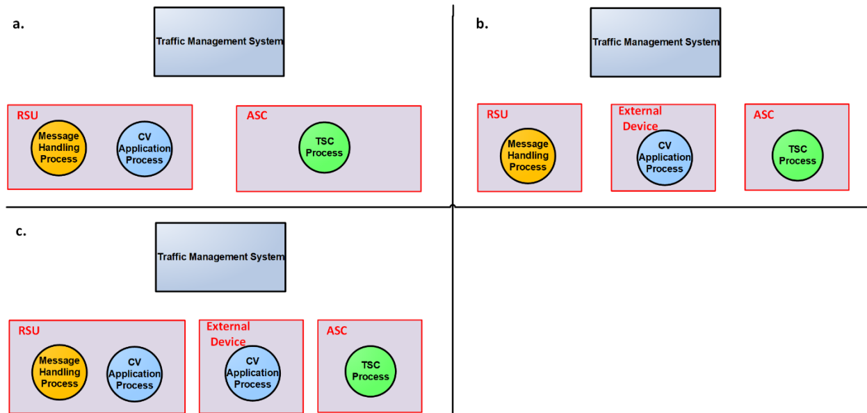
Figure 6 Physical Architecture 2
