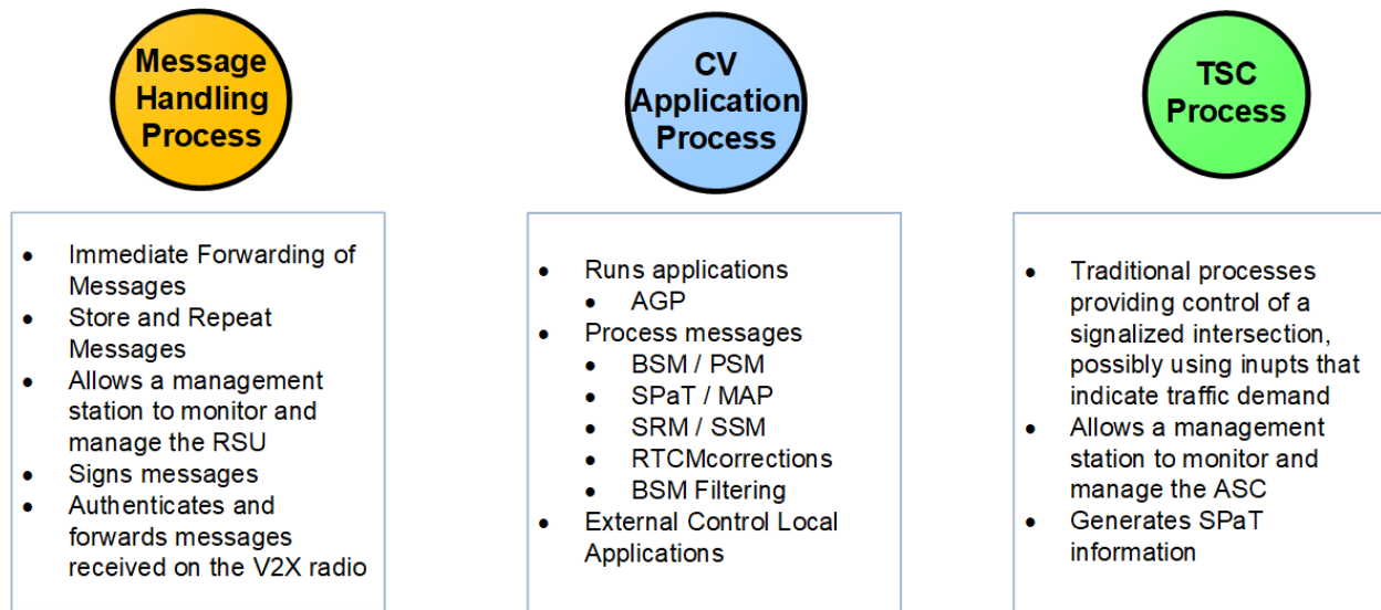
Figure 3 Connected Intersection Logical Processes
