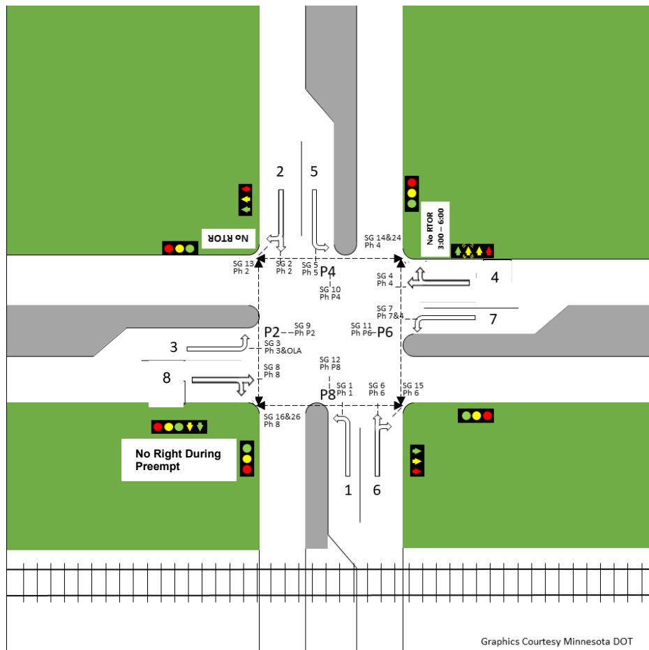
Figure 14 Example Intersection Diagram
