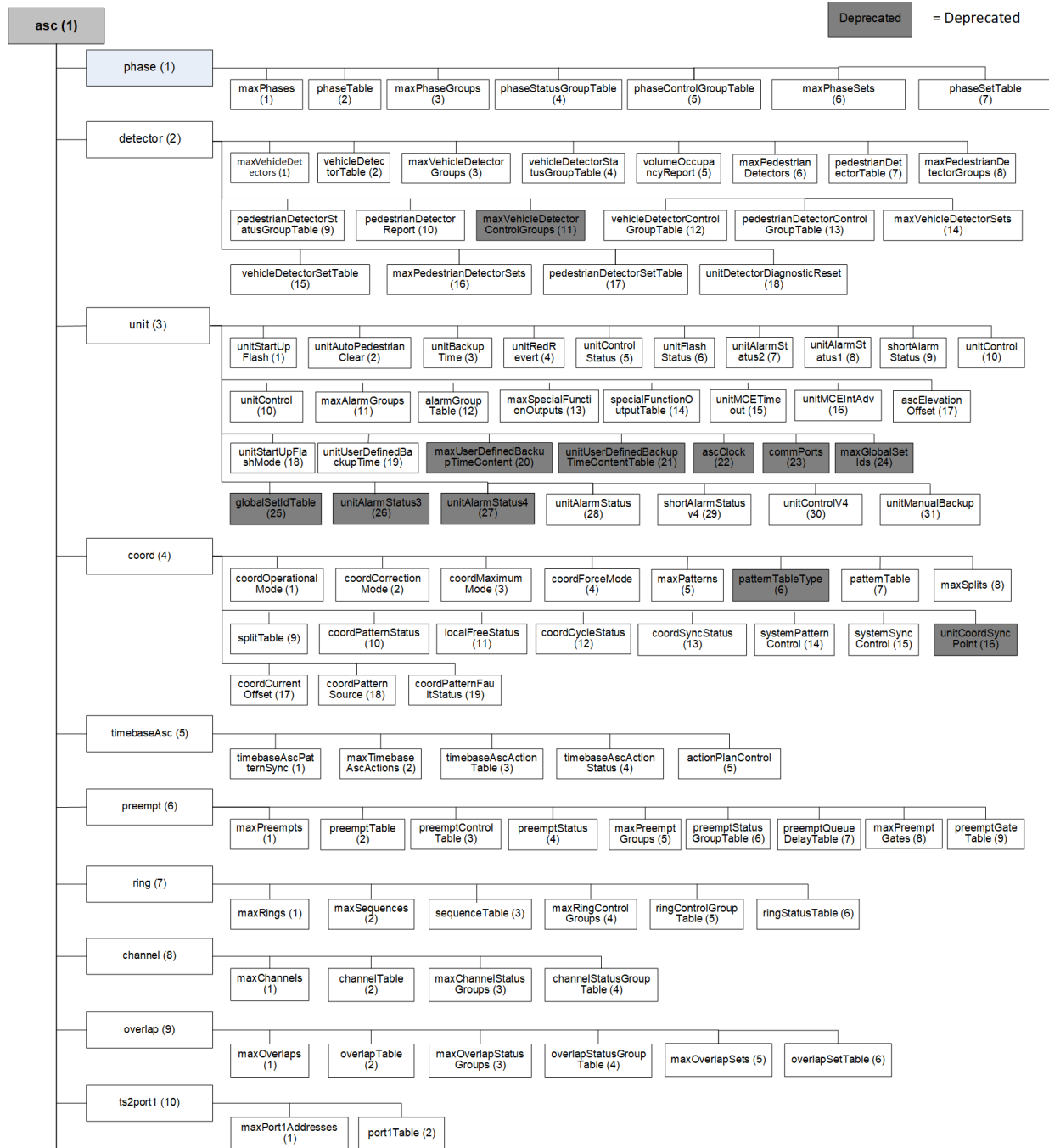
Figure 11 Object Tree for NTCIP 1202 v04 (continued in Figure 12)
