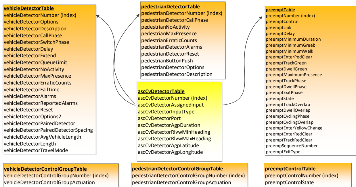
Figure 21 NTCIP 1202 v04 Tables to Receive CV Data
