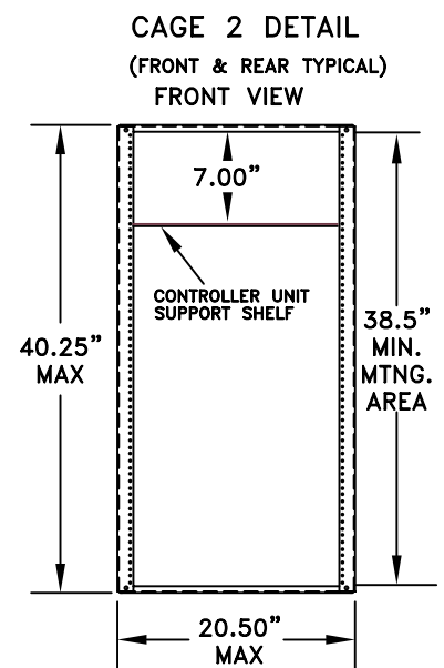
EIA RAIL DIMENSIONS CAGE 2
