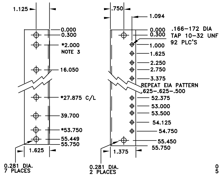
EIA RAIL DIMENSIONS CAGE 1
