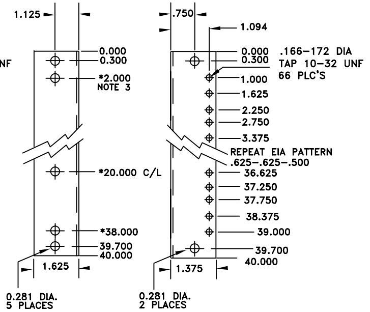
EIA RAIL DIMENSIONS CAGE 2
