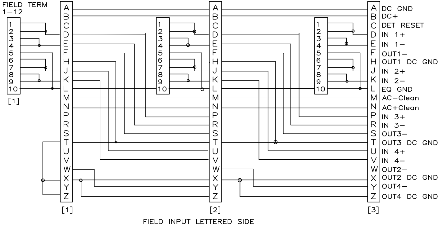
FIELD INPUT LETTERED SIDE
