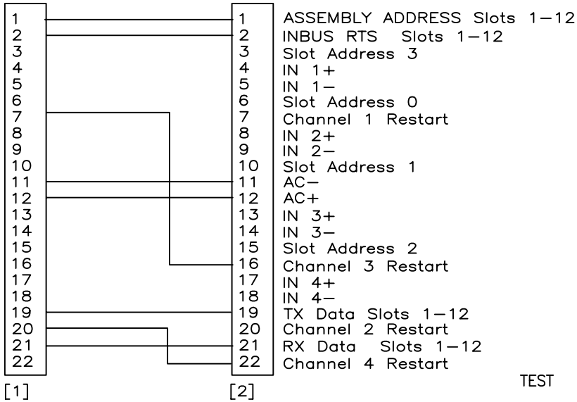
FIELD INPUT CONNECTOR NUMBERED SIDE
