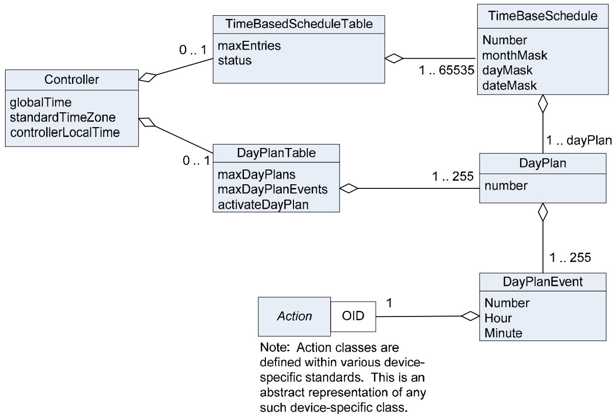
Figure 13 Class Diagram of Generic Schedule-Related Information
