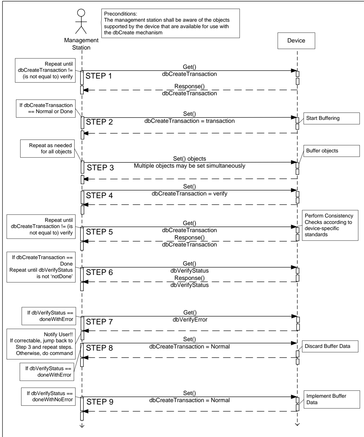
Figure 3 Download Transaction Process Sequence Diagram
