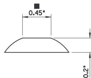
TRUNCATED DOME ELEVATION
